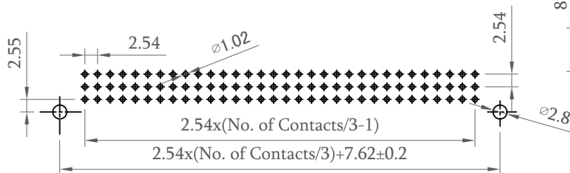
Part No. Pin No. Pitch Rows with Pins Contact Arrange 5DINRL3AXM-96 *** 96 2.54 A B C 5DINRL3BXM-64 *** 64 A B - 5DINRL3CXM-64 *** 64 A - C 5DINRL3DXM-32 *** 32 A - - 5DINRL3EXM-48 *** 48 5.08 A B C 5DINRL3FXM-32 *** 32 A B - 5DINRL3GXM-32 *** 32 A - C 5DINRL3HXM-16 *** 16 A - -
