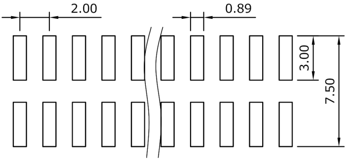
Recommended PCB Layout (PCB TOLERANCE ±0.05)
